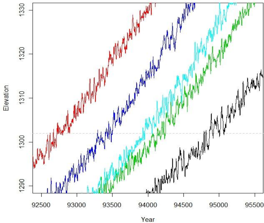
Figure 10. Simulated transgressions of a large lake including short-term variations in lake elevations
