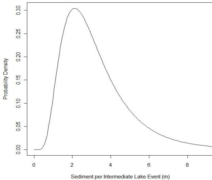
Figure 11. Probability density function for the total sediment thickness associated with an intermediate lake (or the transgressive or regressive phase of a large lake)
