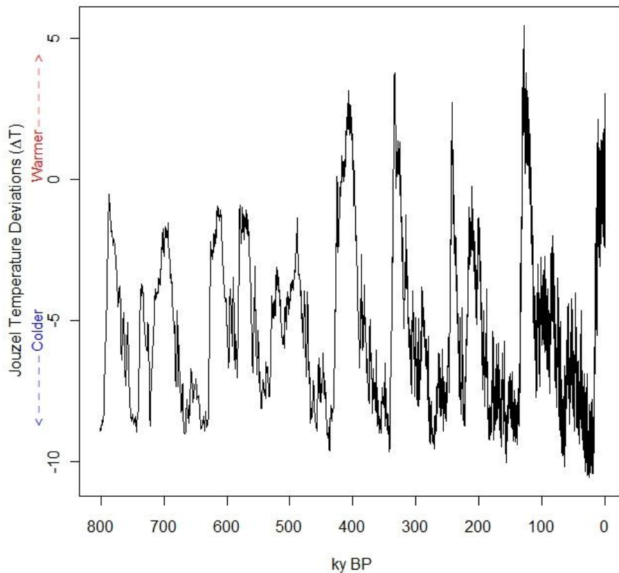
Figure 4. Temperature deviations for the last 810 k (from Jouzel et al. 2007)
