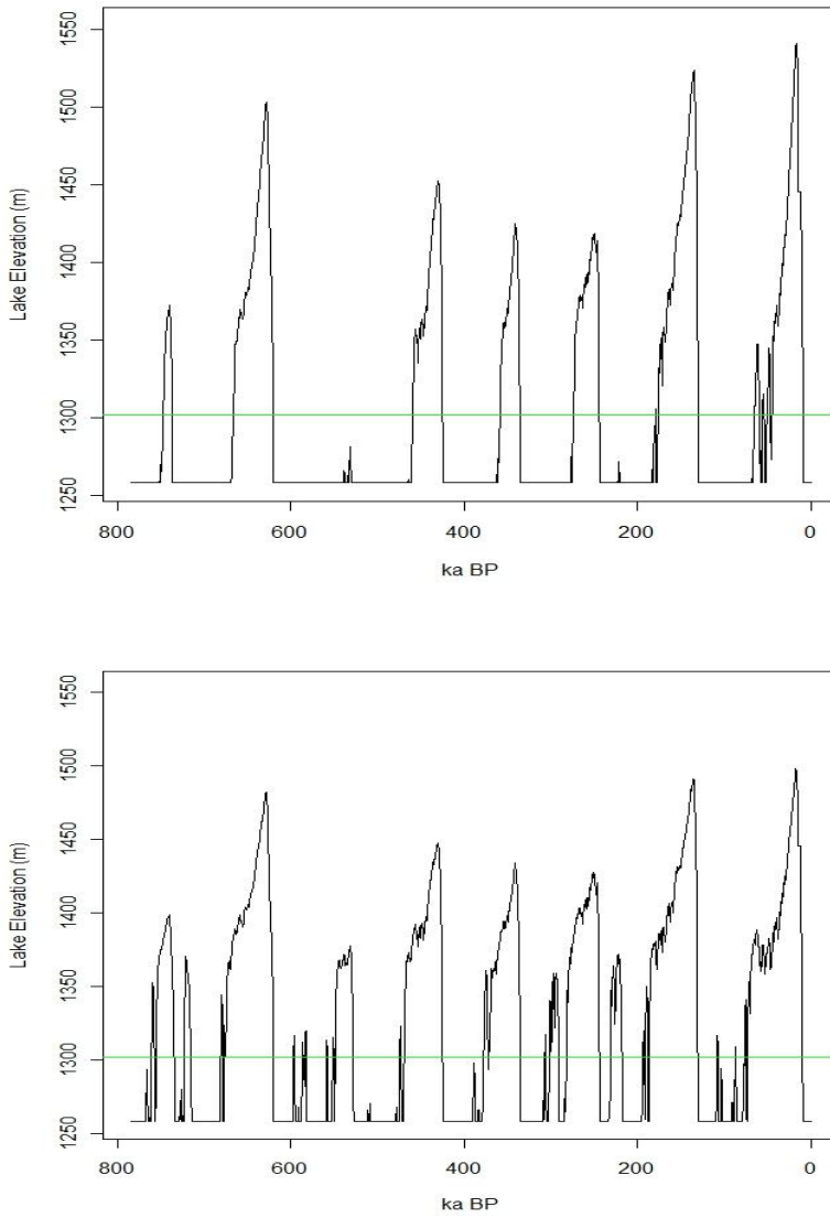
Figure 6. Two example simulated lake elevations as a function of time, with Clive facility elevation represented by green line
