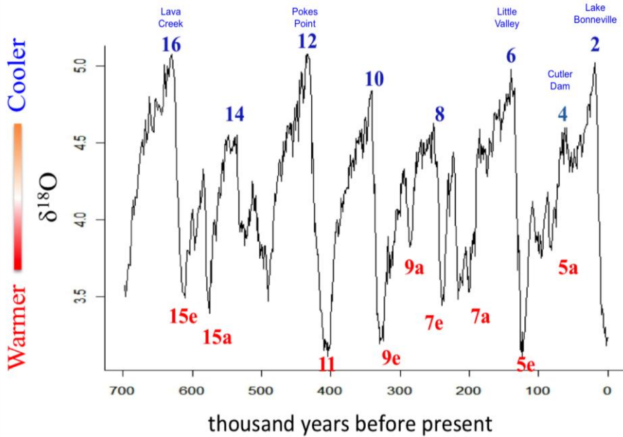
Figure 2. Benthic oxygen isotope record for the last 700,000 years (from Lisiecki and Raymo 2005) 3
