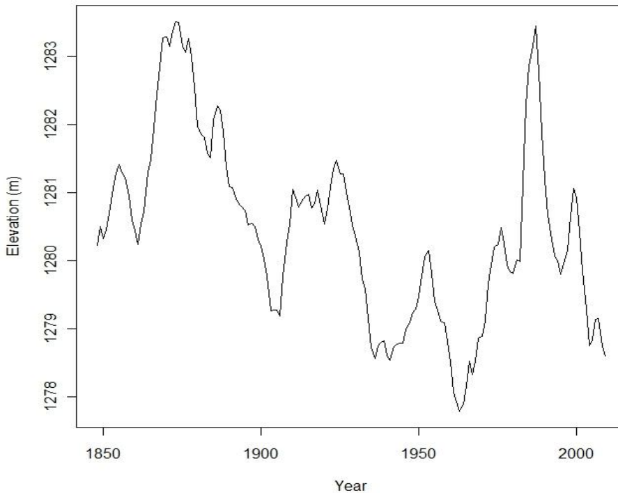
Figure 9. Historical elevations of the Great Salt Lake
