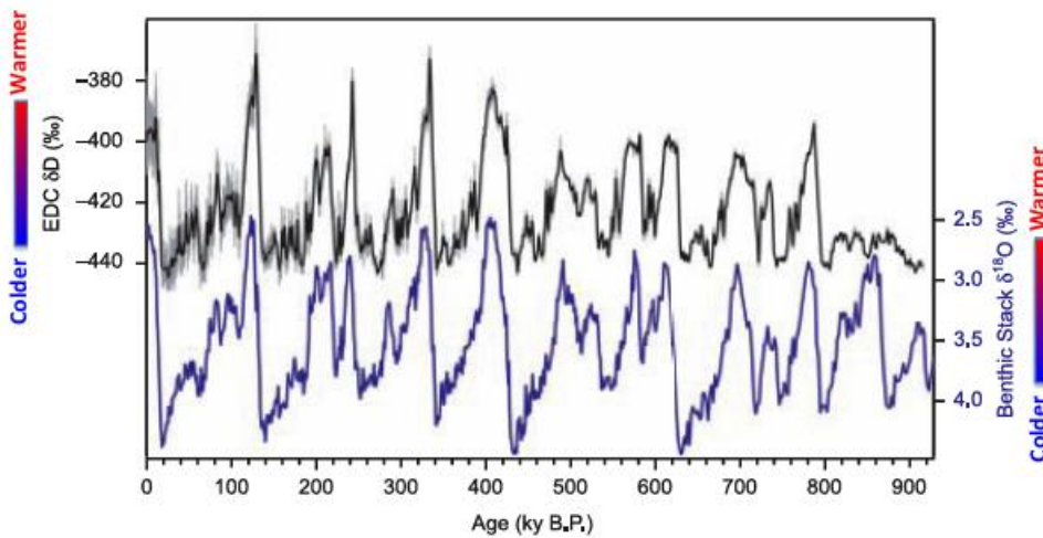
Figure 1. Comparison of delta deuterium (black line) from the European Project for Ice Coring in Antarctica (EPICA) Dome C ice core and benthic (marine) oxygen-18 record (blue line) for the past 900 ky [from Jouzel et al. (2007)]
